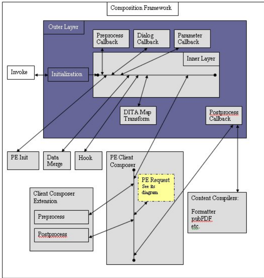
The following diagram illustrates the publishing framework processing of an Arbortext Publishing Engine request on the server.
