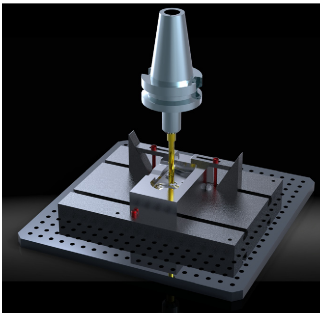
Powerful High Speed Machining toolpaths for core and cavity manufacturing.
