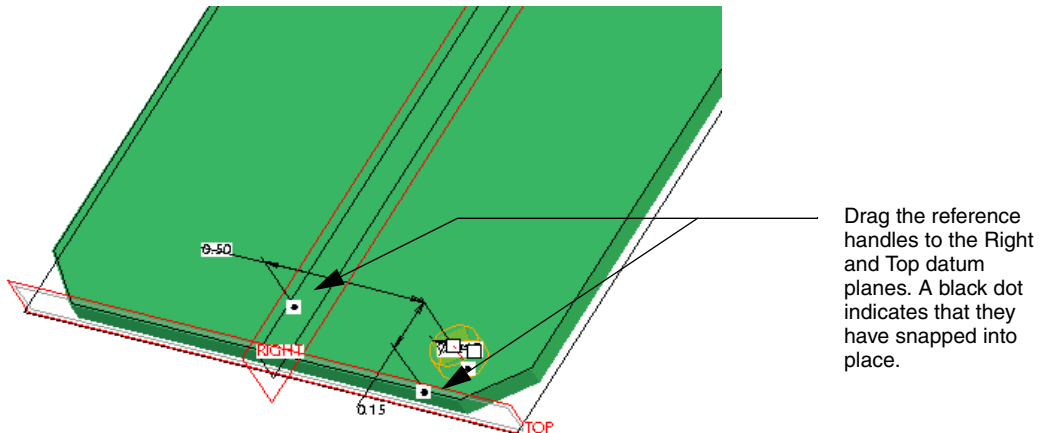
Placing the first hole on the PC board
