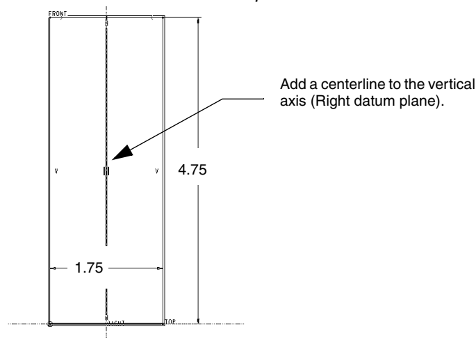
Dimensions for the front cover protrusion
