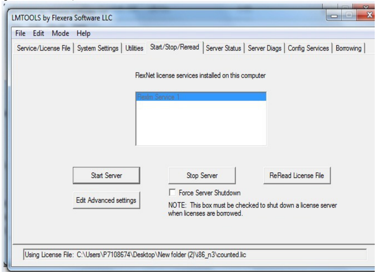
Figure 10-9: Start/Stop/Reread Tab
